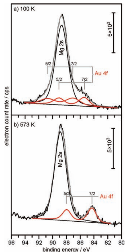
Figure 4. Experimental photoemission spectra and results of fits of the Mg 2s and Au 4f region for 0.02 ML Au (a) deposited at 100 K onto 13 ML MgO hydr(1) and (b) of the same sample after annealing to 573 K.
