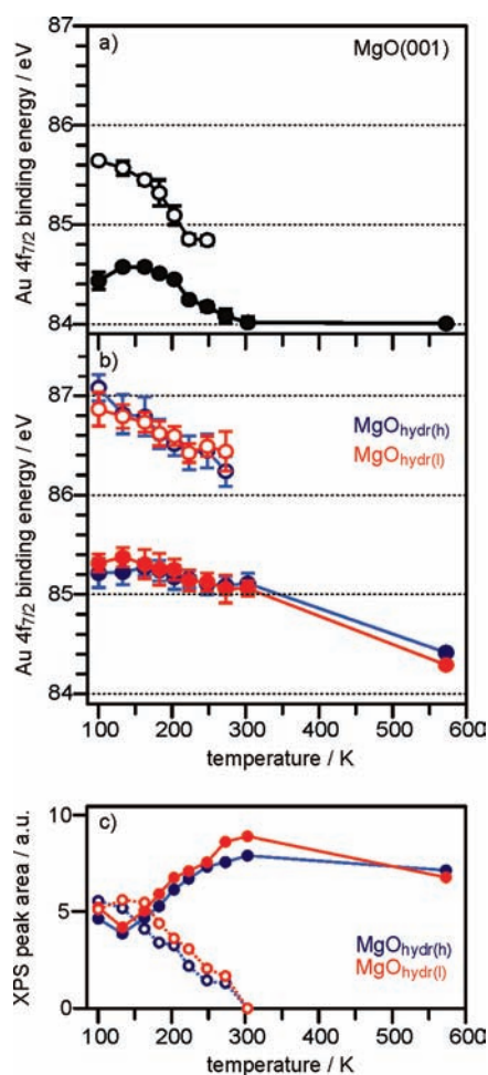
Figure 5. Au 4f_{7/2} binding energies as a function of annealing temperature obtained from fits of the photoemission spectra for 0.02 ML Au deposited at 100 K on (a) 13 ML MgO(001)/Ag(001) and (b) MgO hydr(l) (red) and MgO hydr(h) (blue). (c) Au 4f peak area as a function of annealing temperature for Au/MgO hydr(l) (red) and Au/MgO hydr(h) (blue). Open and solid symbols represent the high and low Au 4f_{7/2} binding energy components, respectively.
