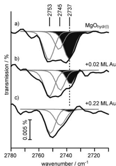
Figure 2. IR spectra taken at room temperature after (a) hydroxylation of 13 ML MgO(001)/Ag(001) at p(\text{D}_2\text{O}) = 1 \times 10^{-3} mbar for 3 min [ \text{MgO}_{\text{hydr}(l)} ], (b) subsequent deposition of 0.02 ML Au, and (c) additional deposition of 0.20 ML Au.
